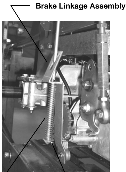
Brake Adjustment Spring
