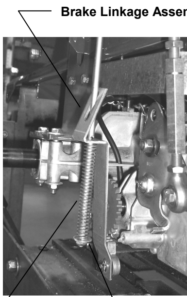
Brake Adjustment Spring Brake Adjustment Nut
